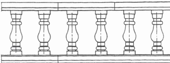
Balusters shown at 305mm centres
